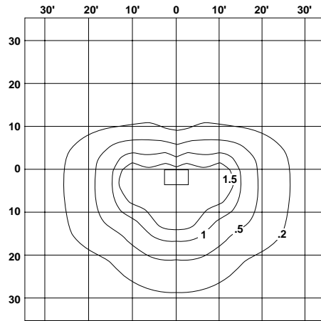
70W HPS Wall Pack at 10' mounting height.
